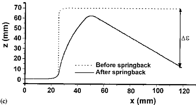
Fig. 6 Simulation results under CBHF of 2.45 kN: (a) forming limited diagram; (b) distribution of engineering thickness strain; (c) profiles before and after springback
