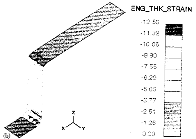
Fig. 7 Forming results under VBHF of 2.45 kN/50 kN: (a) forming limited diagram; (b) distribution of engineering thickness strain
