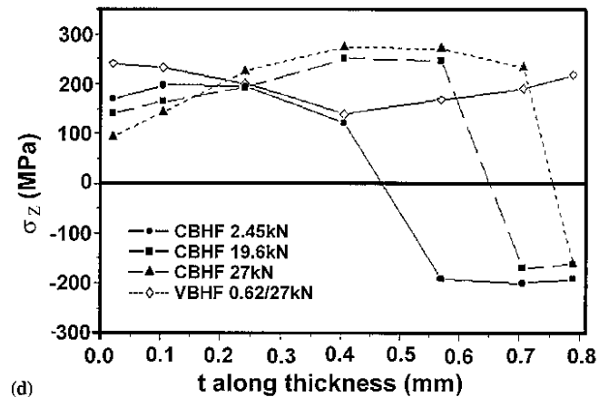
Fig. 12 Tangential stress distributions through the thickness on sidewall: (a) position of measure points; (b) point A; (c) point B; (d) point C
