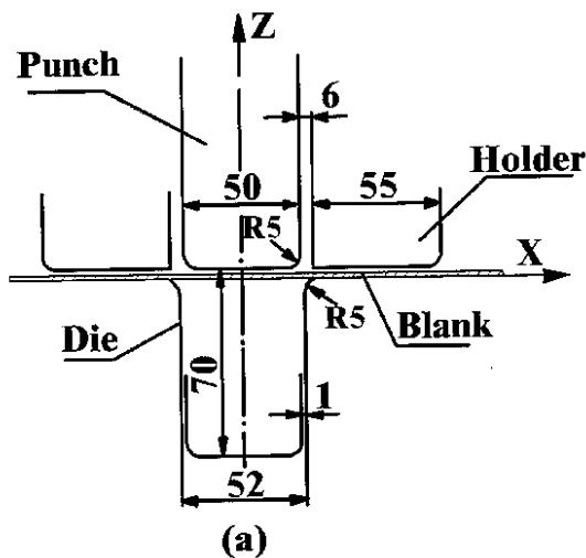
Fig. 4 2-D draw bending problem of NUMISHEET'93: (a) geometry; (b) measuring method
