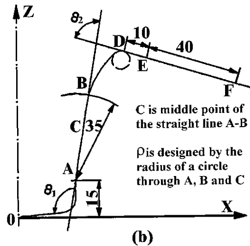
Fig. 4 2-D draw bending problem of NUMISHEET'93: (a) geometry; (b) measuring method
